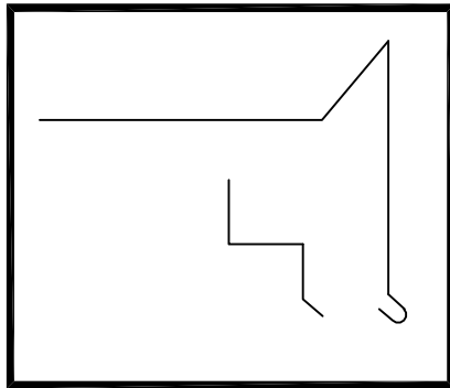
FLASHING COMPONENTS
