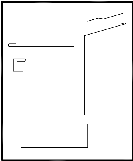
FLASHING COMPONENTS
