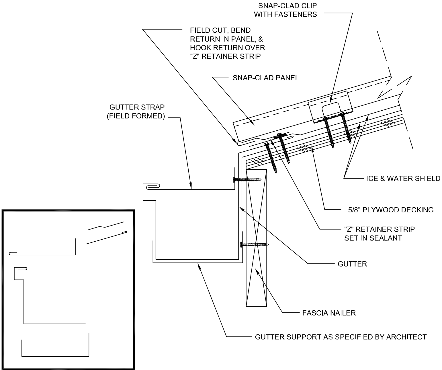
FLASHING COMPONENTS
