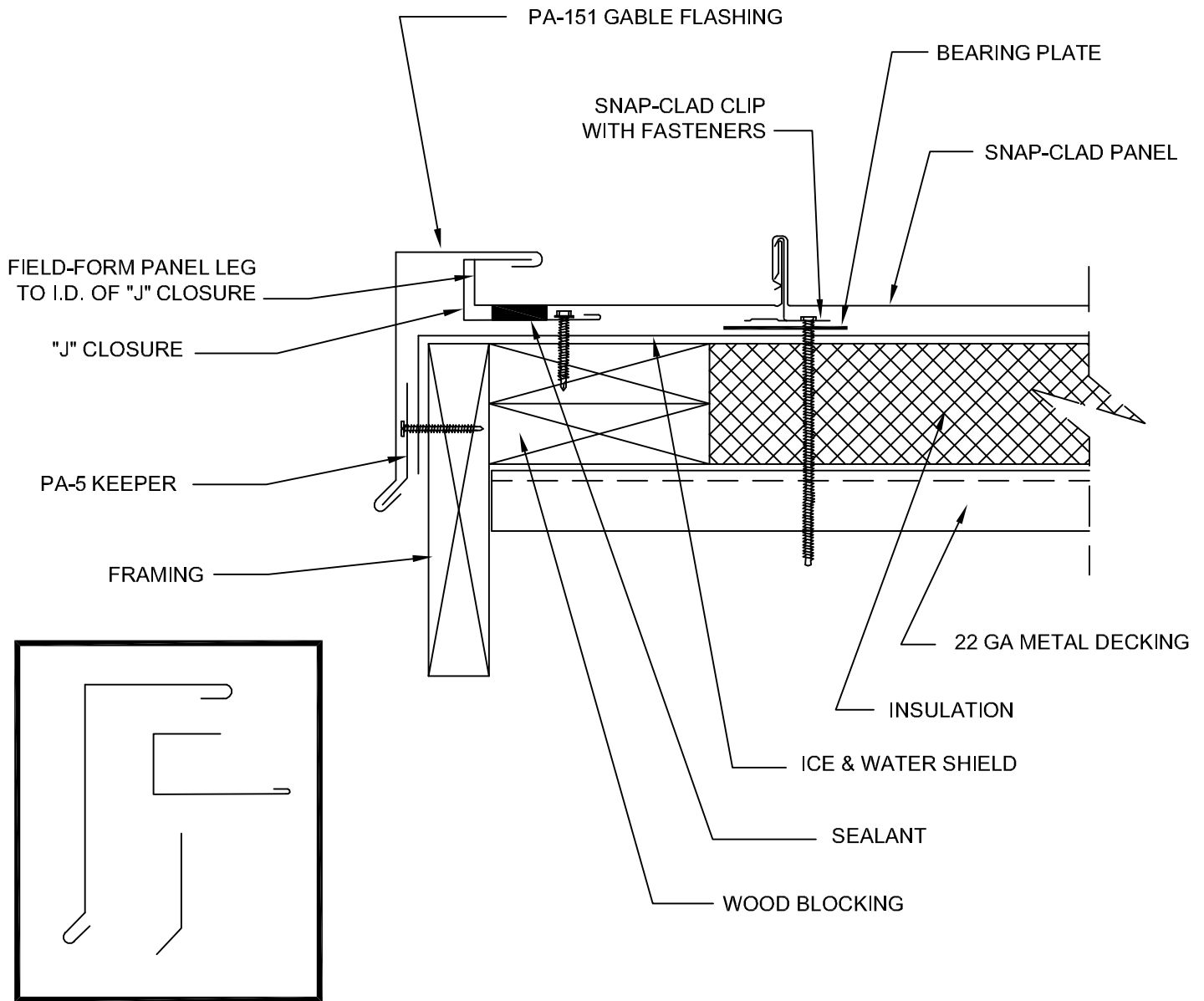
FLASHING COMPONENTS
