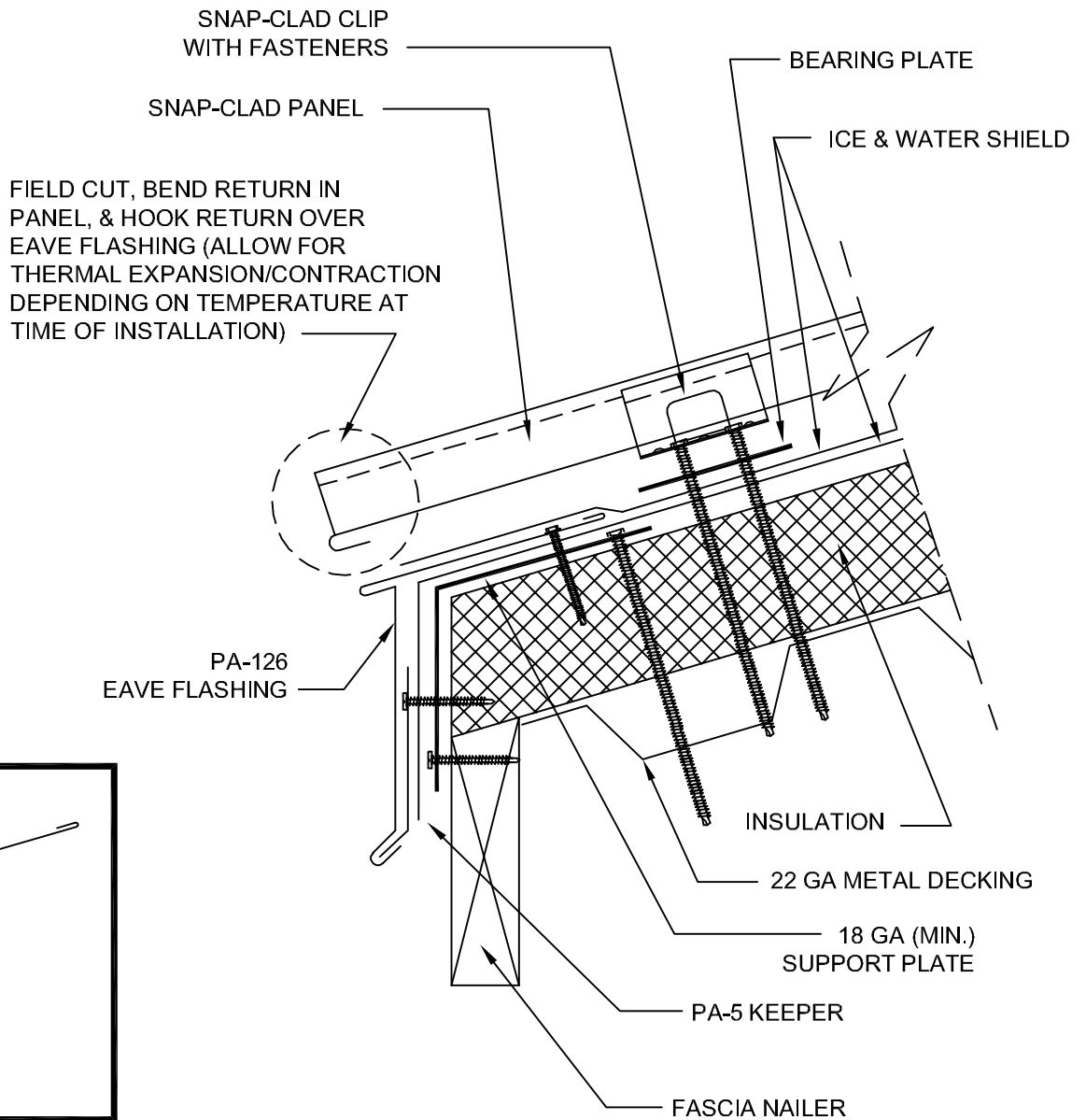
FLASHING COMPONENTS
