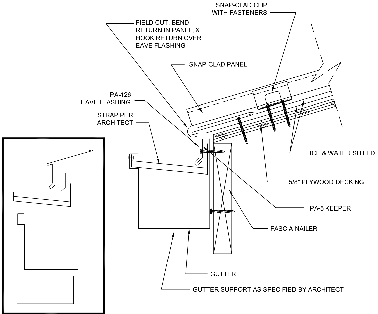
FLASHING COMPONENTS
