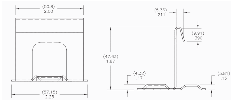
INDIVIDUAL PANEL CLIP
