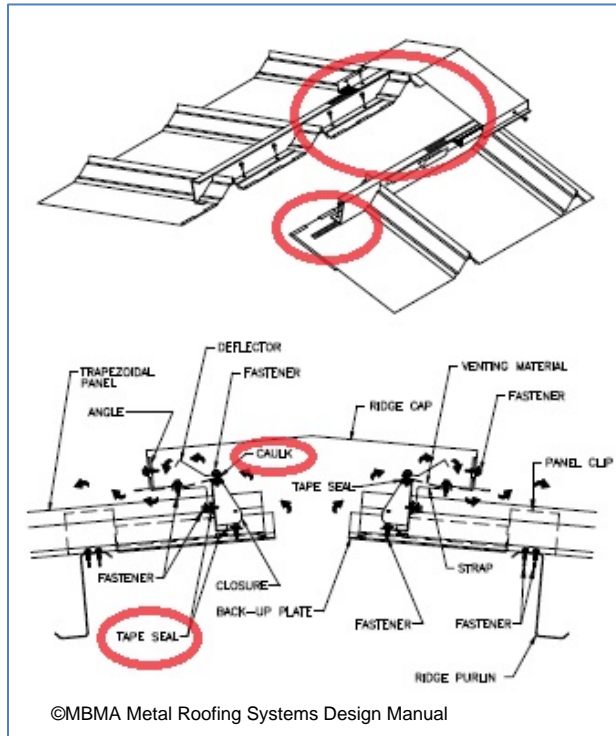
Figure 13-14 Trapezoidal Vented Ridge Sealing Example
