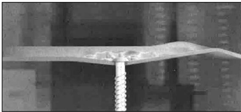
Figure 10-39 Over-Driven Fastener
