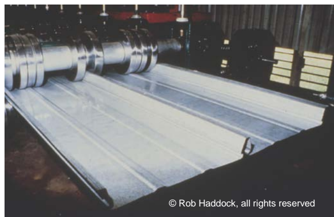
Figure 2-8 Roll Forming Equipment
