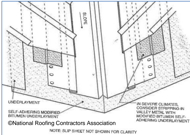
Figure 10-69 Stripping of Nailed Valley Trim
