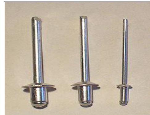
Figure 12-9 Blind Rivets
